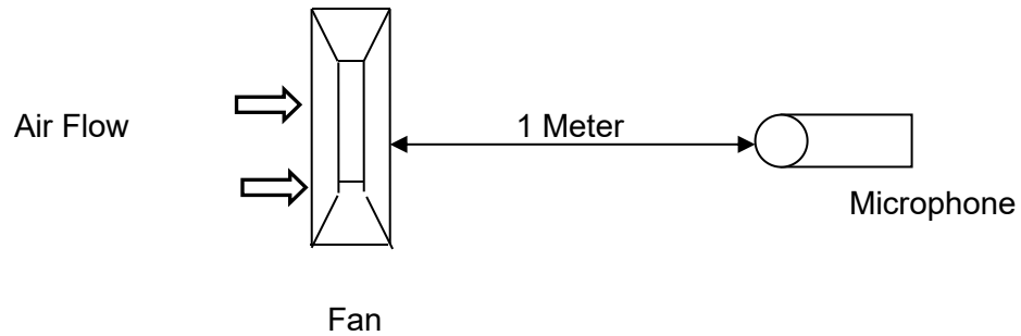
Figure B– Noise Level is measure at rated voltage in an anechoic chamber in free air with reverse blade impeller as above.
